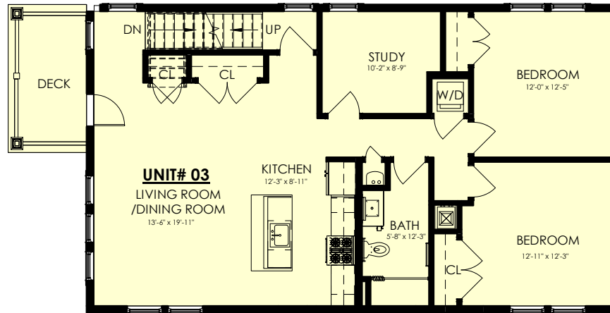
SECOND LEVEL
